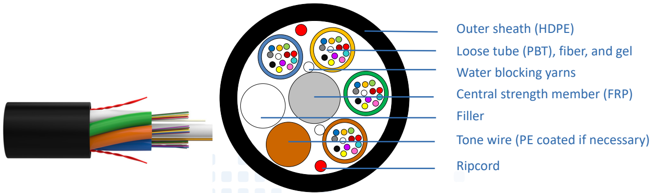
Fig. 1 For 12&14AWG tone wire
